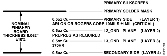
Figure 27. 4-Layer Stackup
