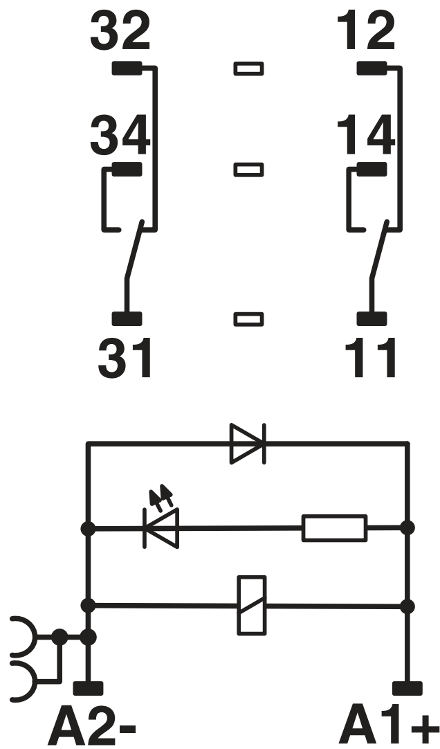
Circuit diagram
