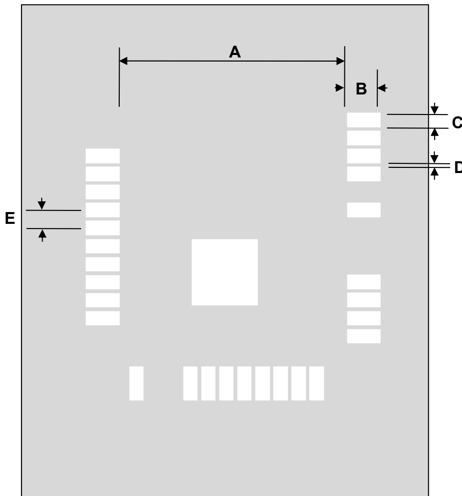
Top View (SMT Footprint)
