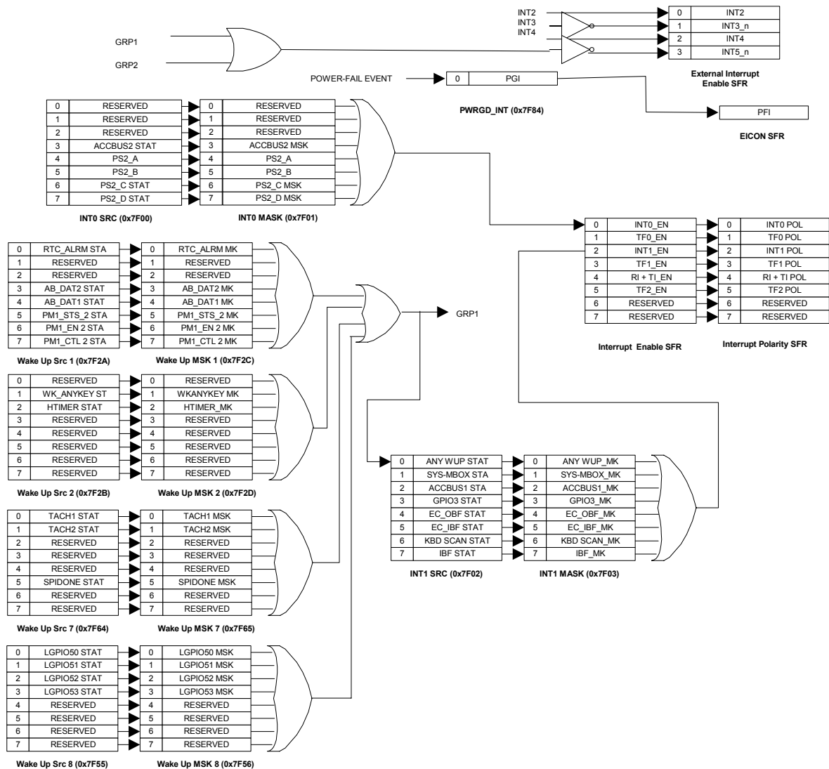
Figure 7.4 8051 Interrupts
