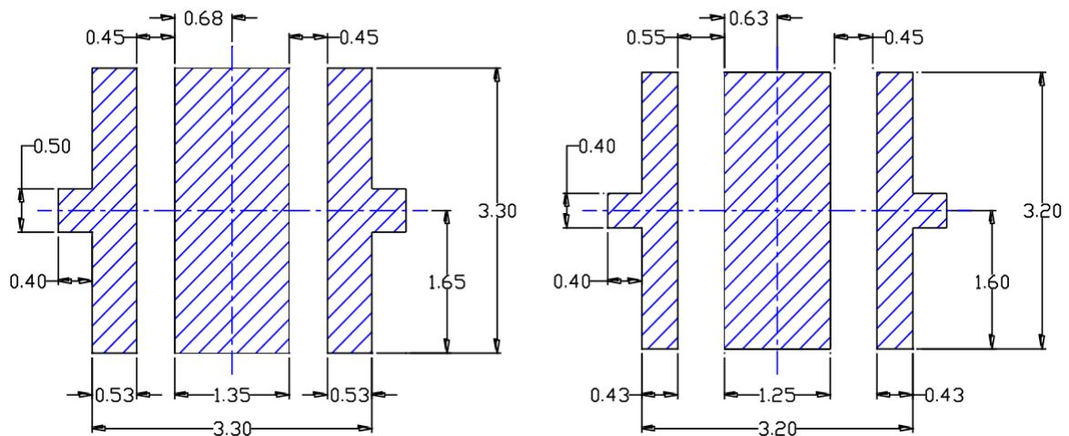
Figure 1. IN-C39ATKU1 / IN-C39BTKU1 / IN-C39CTKU1 Recommended Solder Pattern
