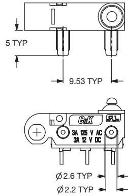
POSTS LEFT MODEL SHOWN: ZMSMHXXXXP00PLC
