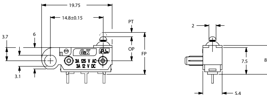
MODEL SHOWN: ZMSMHXXXP00PLC
