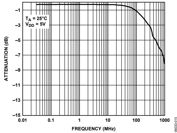
Figure 15. Bandwidth
