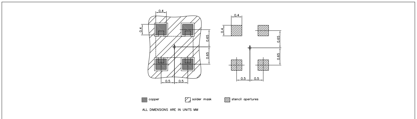
Figure 21 Foot print
