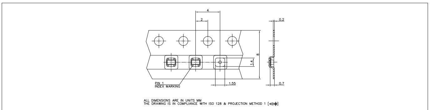
Figure 23 Tape dimensions
