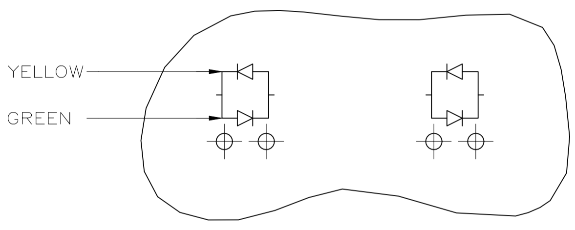
LED CURRENT DIAGRAM 406549-8, 2-406549-8
