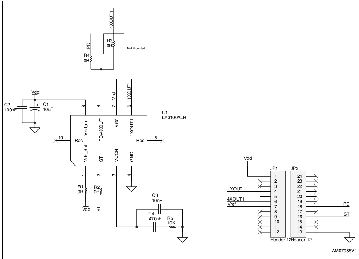
Figure 1. Circuit schematic
