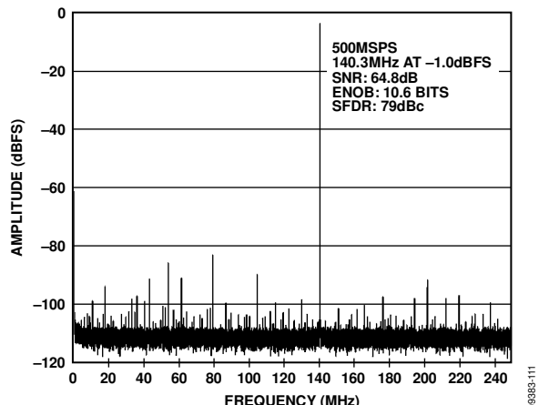
Figure 11. AD9434-500 64k Point Single-Tone FFT; 500 MSPS, 140.3 MHz
