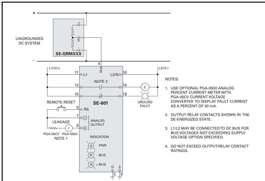
FIGURE 2. Typical Connection Diagram.
