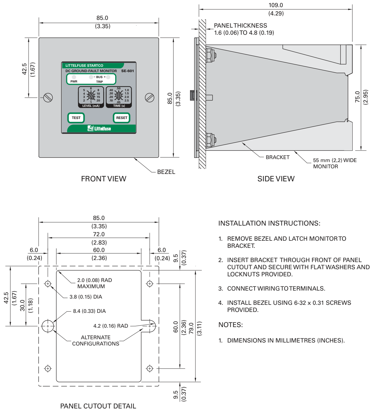
FIGURE 6. PMA-55 Panel-Mount Adapter.
