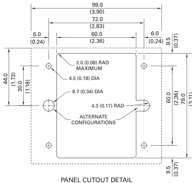
FIGURE 7. PMA-60 Panel-Mount Adapter.
