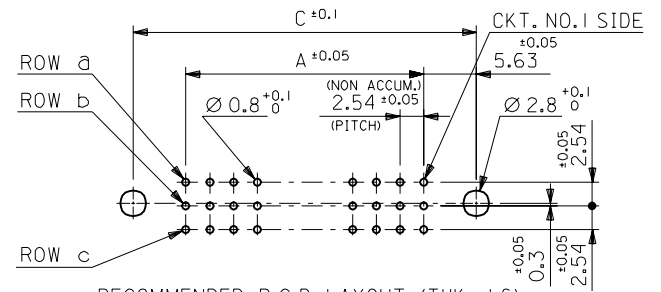
RECOMMENDED P.C.B. LAYOUT (THK.=1.6) (VIEW ON COMPONENT SIDE)
