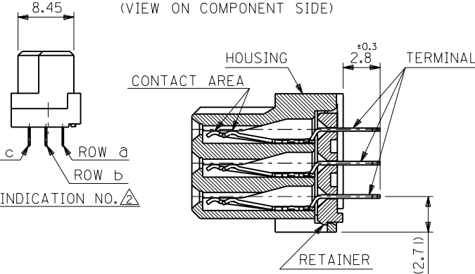
SECT. Z-Z (SCALE:4-1)
