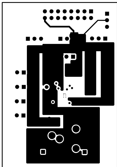
Figure 43. Layer 2
