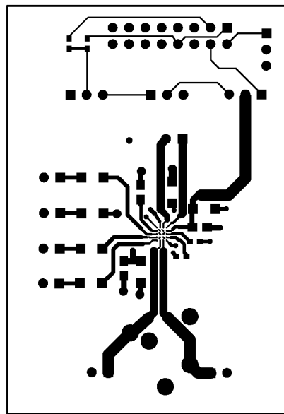
Figure 42. Top Layer
