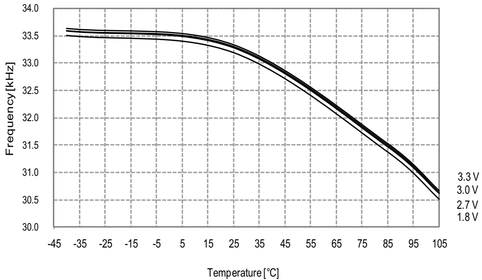
Figure 33-54. Ultra Low-power Internal Oscillator Frequency vs. Temperature
