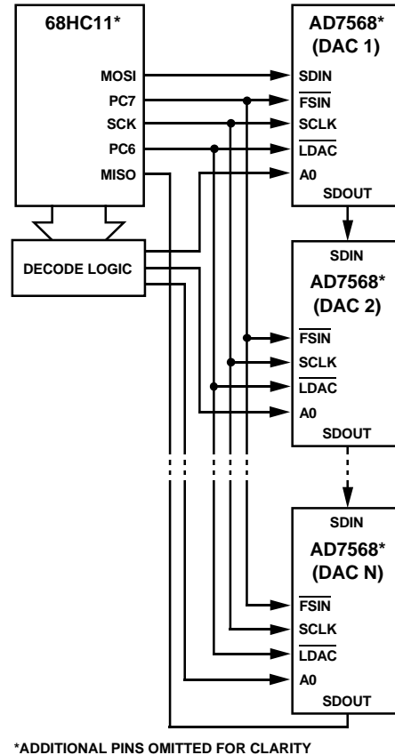
Figure 25. Multi-DAC System
