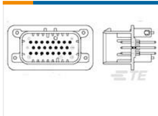
TE Part #776231-1 35POS, PIN DIA 1.3, HDR ASSY, 180DEG, COD 1
