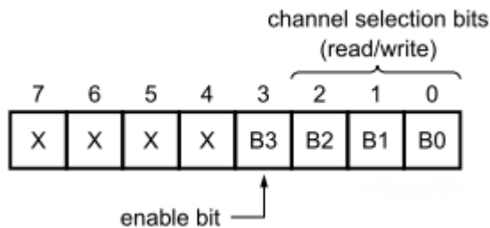
Figure 5: Control register
