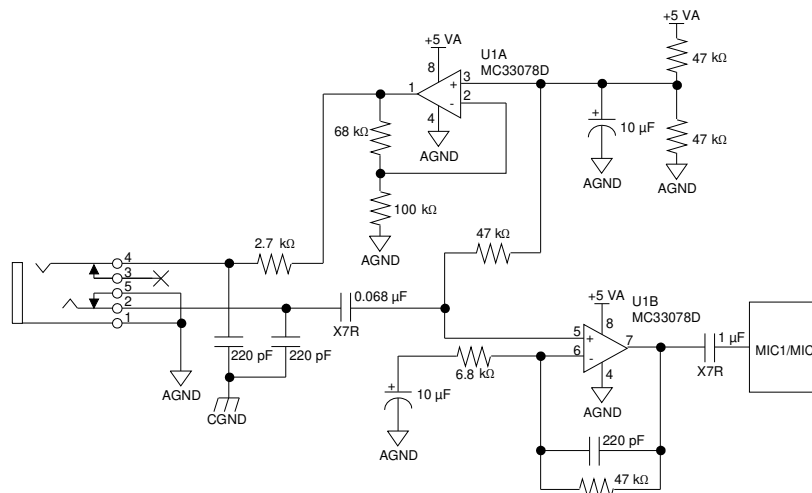
Figure 6-4. Microphone Pre-amplifier
