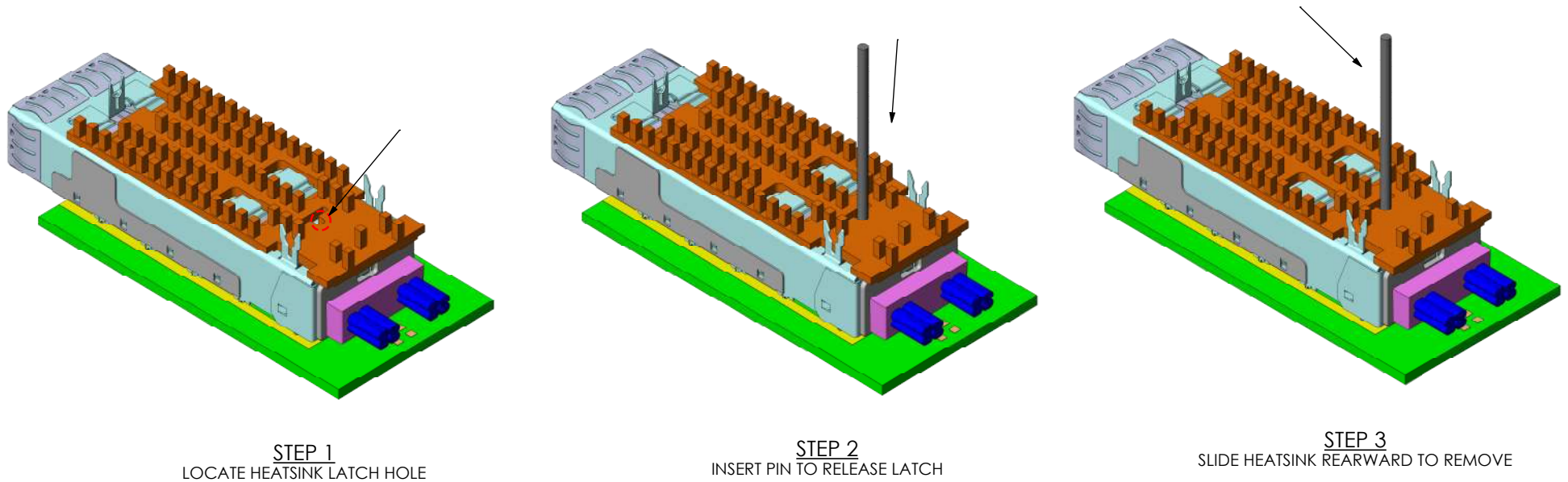
FIG 15 HEAT SINK REMOVAL
