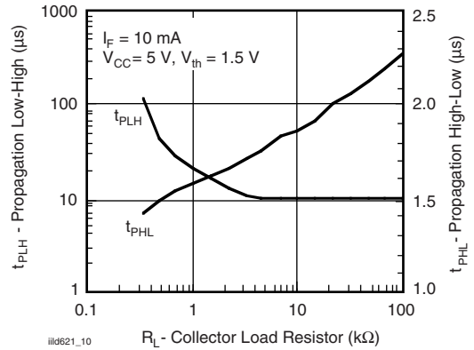
Fig. 10 - Propagation Delay vs. Collector Load Resistor
