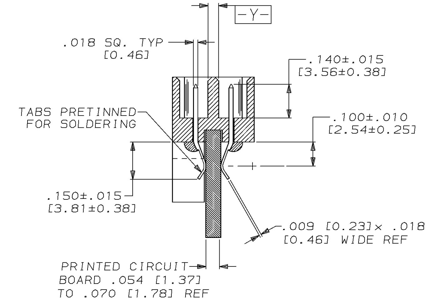
SECTION T-T
