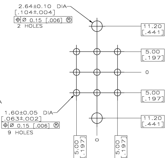
RECOMMENDED LAYOUT
