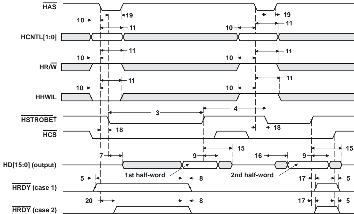
Figure 28. HPI Read Timing (HAS Used)
