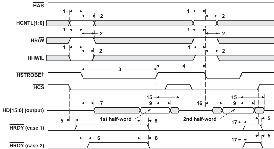
Figure 27. HPI Read Timing (HAS Not Used, Tied High)
