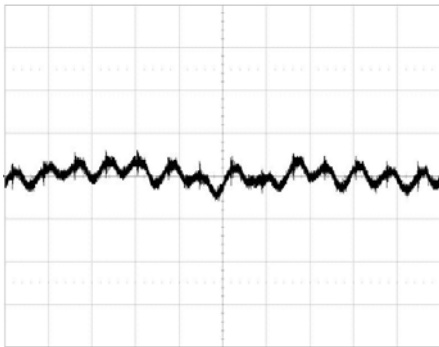
Output voltage ripple (5 mV/div.) at: T_{ref} = +25^{\circ}C , I_O = 60 A electrical load, V_I = 5 V . Time scale: 5 \mu s /div. Output capacitor: 660 \mu F electrolysis type. See the filter in the Output ripple and noise section (EMC Specification).
