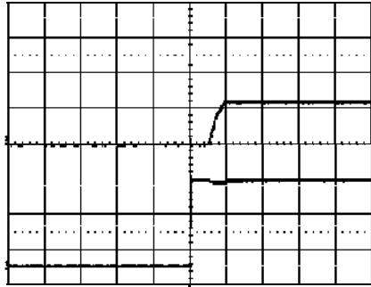
Start-up enabled by connecting V_I at: T_{ref} = +25^{\circ}C , I_O = 60 A resistive load, V_I = 5.0 V . Top trace: output voltage (1.0 V/div.). Bottom trace: input voltage (2.0 V/div.). Time scale: 10 ms/div.
