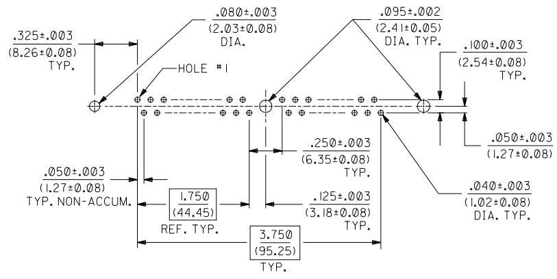
RECOMMENDED SOCKET P.C. BOARD HOLE PATTERN
