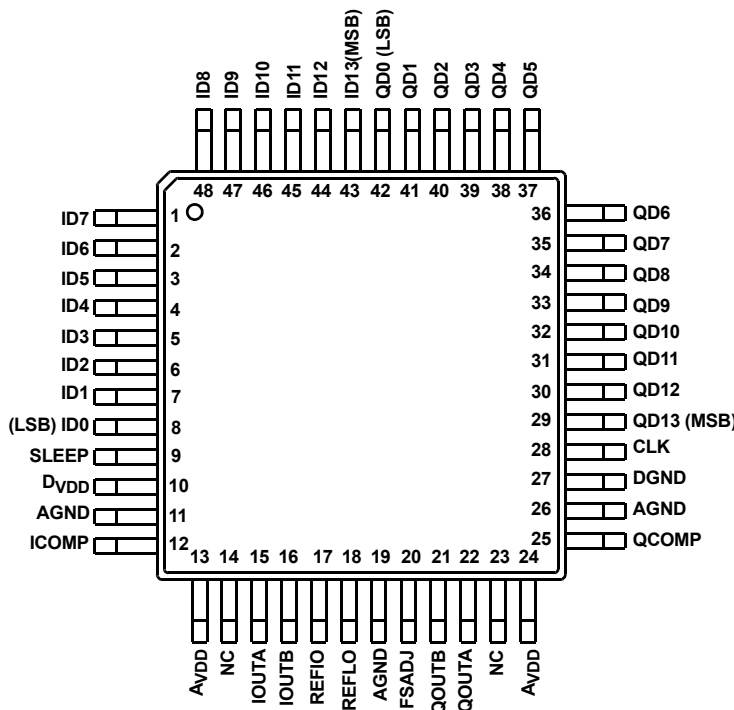
ISL5929 (LQFP) TOP VIEW
