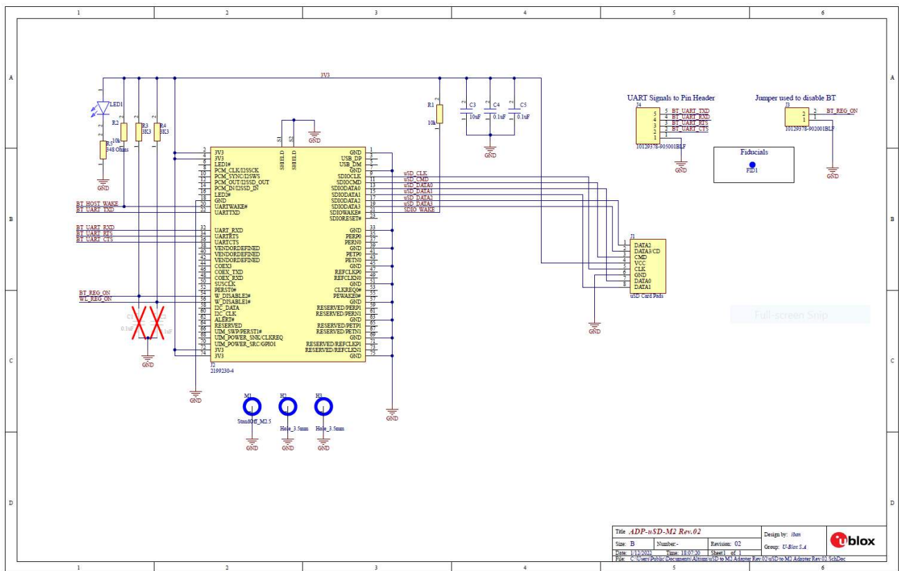
Figure 3: ADP-uSD-M2 schematic
