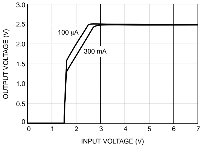
Figure 3. Dropout Characteristics
