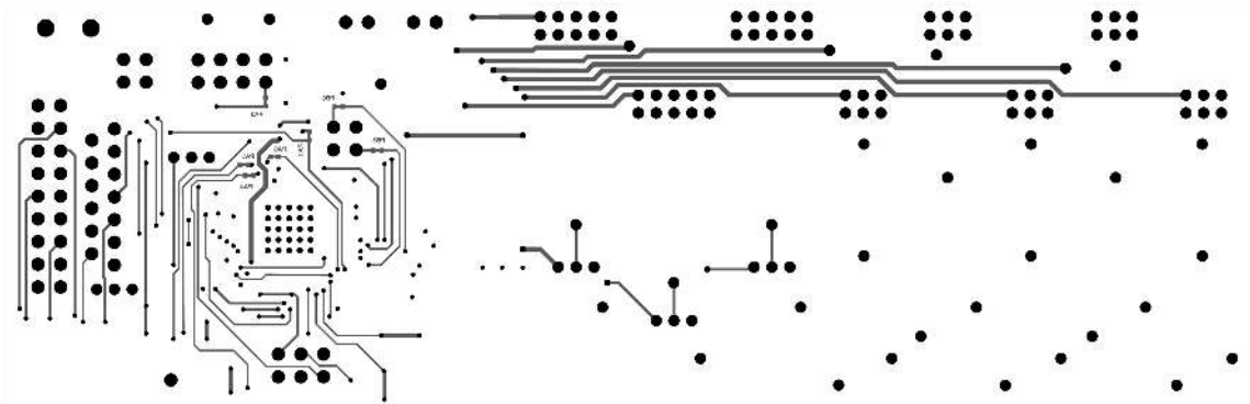
Figure 9-9. Atmel ATAB664251A Board; Bottom Side, Top View (as if PCB is Transparent)
