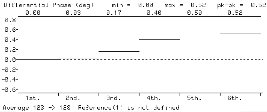
Figure 10. Differential Phase
