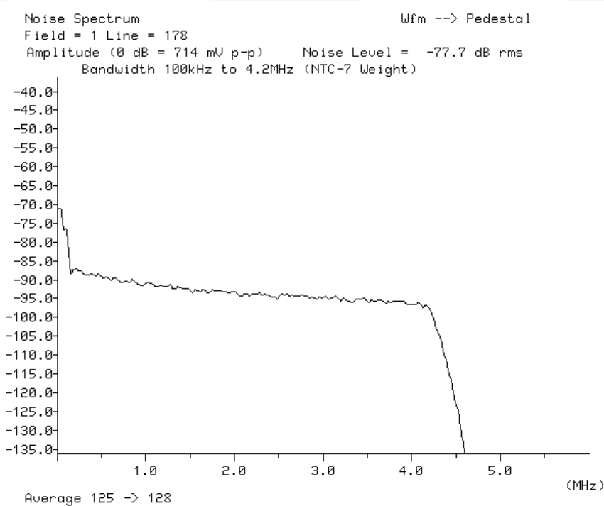
Figure 6. Noise vs. Frequency
