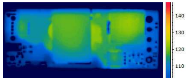
Figure 6. Thermal Image of CPE10A48 (10A output, 70C Ambient, 100lfm airflow, Vin = 48V, airflow from pin 3 to pin 1, T max = 119°C)
