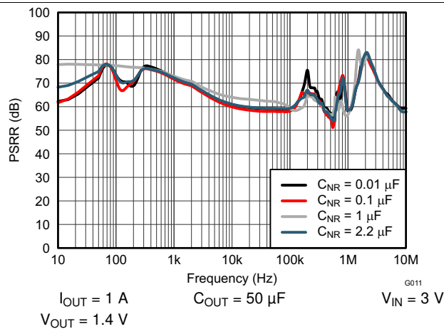
Figure 11. Power-Supply Rejection Ratio vs C_{\text{NR}}
