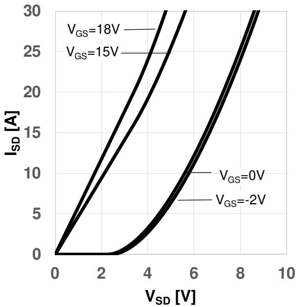
Figure 13 Typical body diode forward current as a function of forward voltage, V_{GS} as parameter ( I_{SD} = f(V_{SD}) , T_{vj} = 25^{\circ}C , t_P = 20\mu s )
