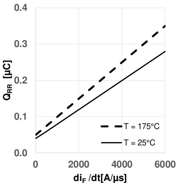
Figure 19 Typical reverse recovery charge as a function of diode current slope (Q_{rr} = f(di_i/dt), V_{DD} = 800V, V_{GS} = 0V/18V, I_D = 4A, \text{ind. load, test circuit in Fig.E, body diode at } V_{GS} = 0V)
