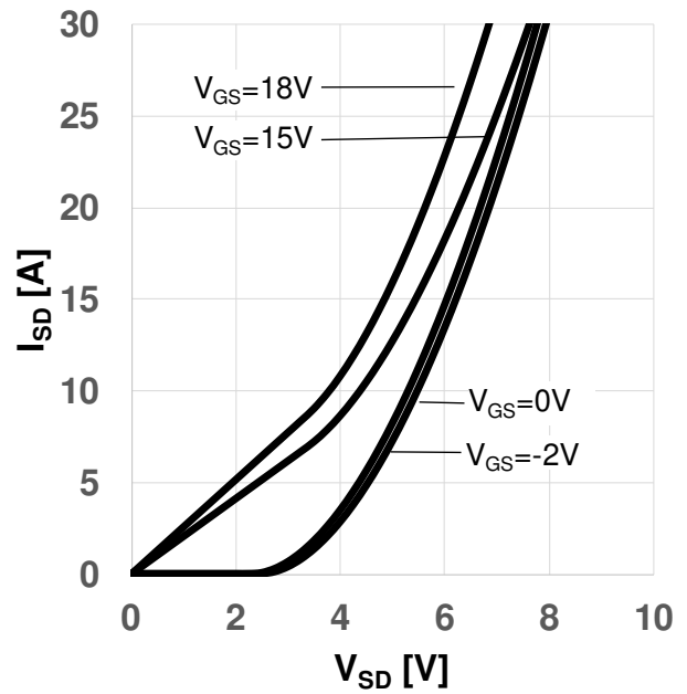
Figure 14 Typical body diode forward current as a function of forward voltage, V_{GS} as parameter ( I_{SD} = f(V_{SD}) , T_{vj} = 175^{\circ}C , t_P = 20\mu s )
