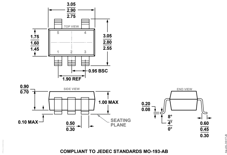
COMPLIANT TO JEDEC STANDARDS MO-193-AB Figure 47. 5-Lead Thin Small Outline Transistor Package [TSOT] (UJ-5) Dimensions shown in millimeters
