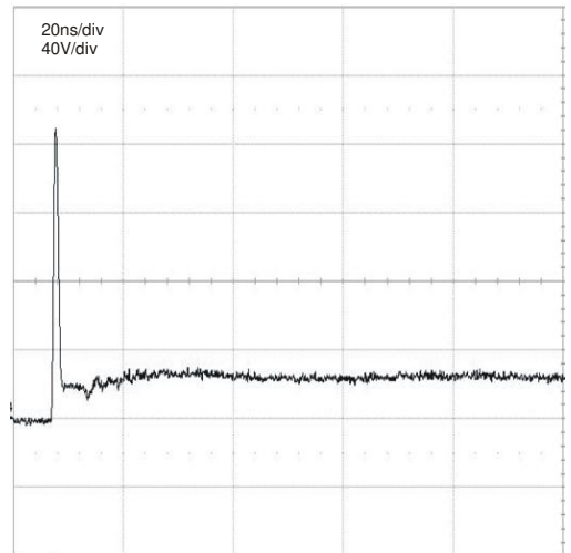
Figure 6 ESD Response to IEC 61000-4-2 (+8kV Contact Discharge)
