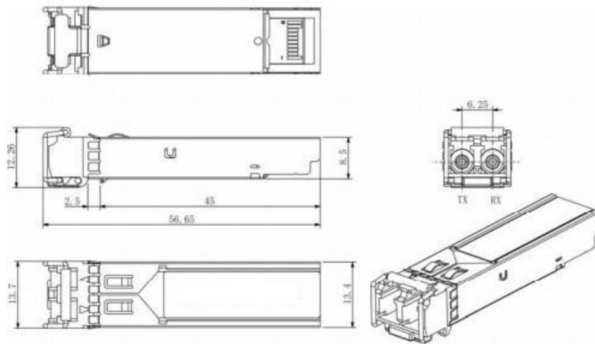
Mechanical Drawing
