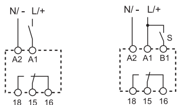
Wiring diagram (without control signal) Wiring diagram (with control signal)
