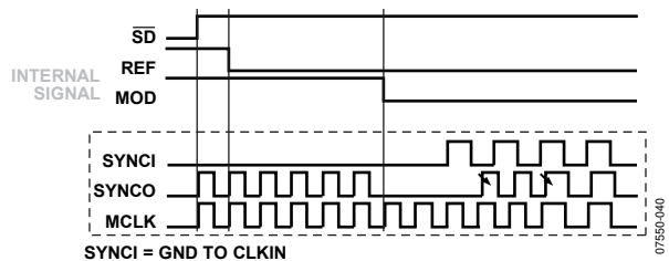
Figure 40. SYNCI = GND to Clock Input
