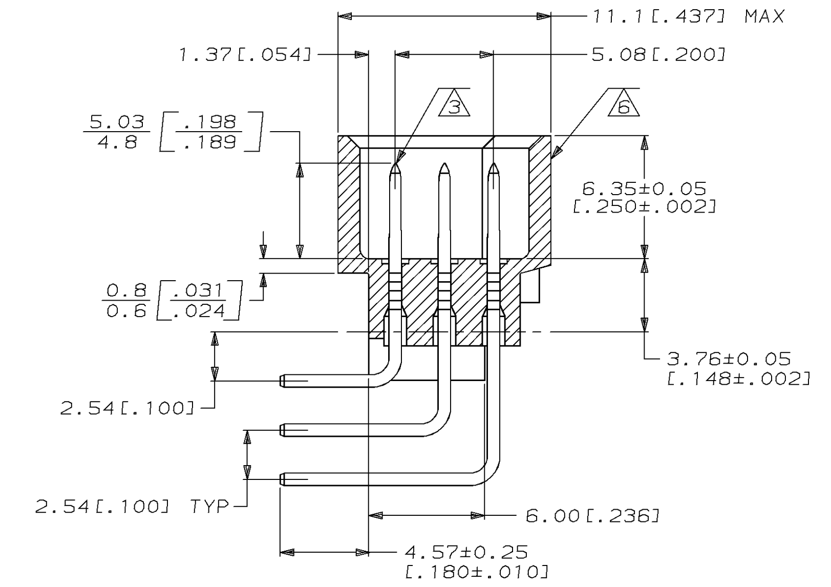
SECTION Z-Z
