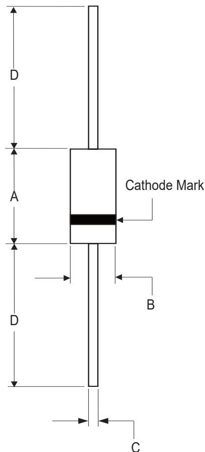
DO-201AE
