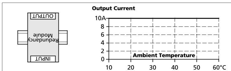
Fig. 17-5 Mounting Orientation B (Upside down)
