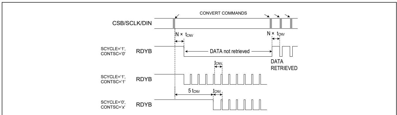
Figure 4. Timing of RDYB in All Conversion Configurations: Single-Cycle, Single-Cycle Continuous and Continuous. In sequencer mode 1 and in sequencer modes 2 and 3, with SEQ:RDYBEN=0' N = 1. In sequencer modes 2 and 3 with SEQ:RDYBEN=1' N = number of active channels.
