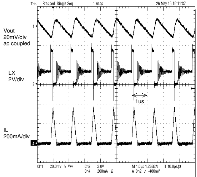
Figure 66. PFM mode Operation Iout=50mA
