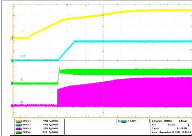
Figure 8-14. Start-Up Relative to VIN
