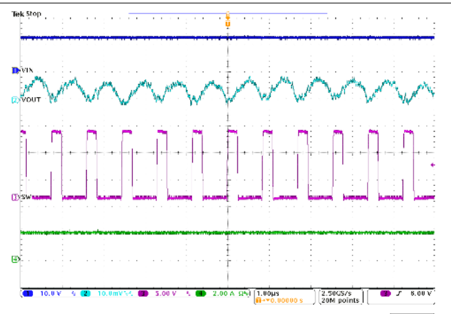
Figure 8-9. Steady State Waveforms, I_{OUT} = 2\text{ A}
