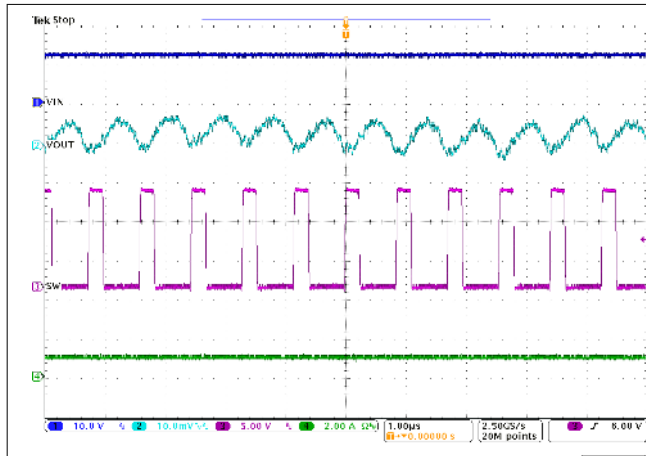
Figure 8-8. Steady State Waveforms, I_{OUT} = 1.0\text{ A}
