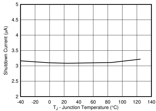
Figure 6-3. Shutdown Current vs Junction Temperature
