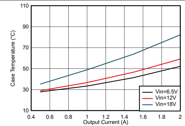
Figure 8-5. Case Temperature Rise vs Load Current
