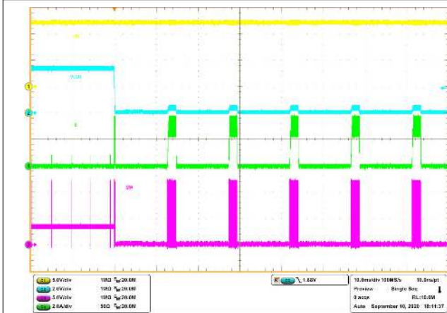
Figure 8-18. Output Short Protection (ECO)
