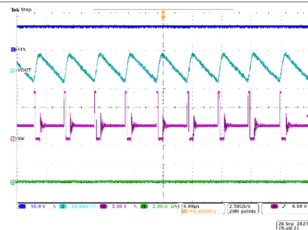
Figure 8-7. Steady State Waveforms, I_{OUT} = 0.1\text{ A}
