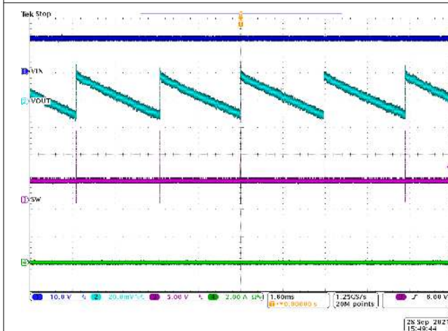
Figure 8-6. Steady State Waveforms, I_{OUT} = 0\text{ A}
