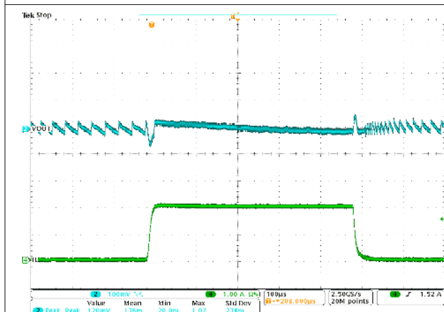
Figure 8-12. Transient Response 0 to 2 A with Slew Rate of 2.5 A/ \mu\text{s} (ECO)
