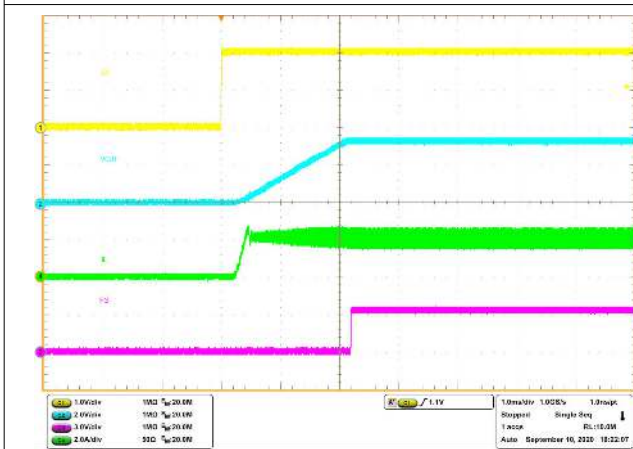
Figure 8-16. Enable Relative to EN
