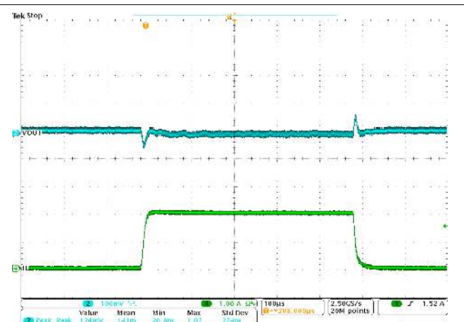
Figure 8-13. Transient Response 0 to 2 A with Slew Rate of 2.5 A/ \mu\text{s} (FCCM)
