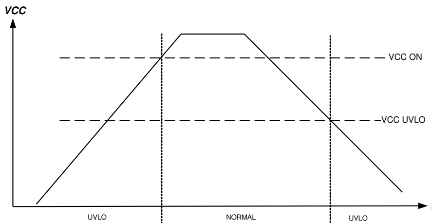
Figure 11: Vcc UVLO
