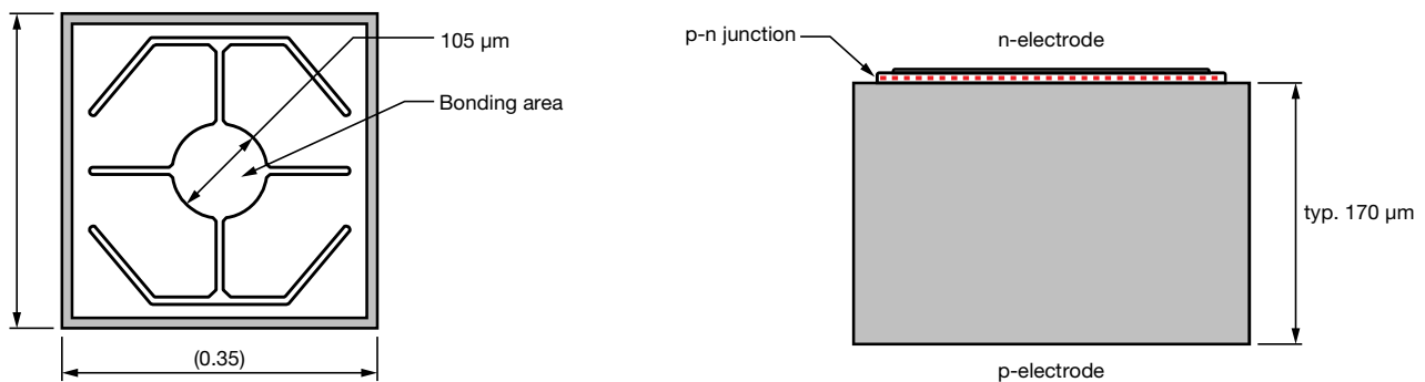
Fig. 3 - Sectional View
