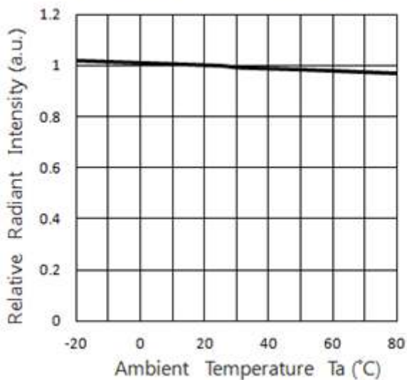
Fig.3-Relative Radiant Intensity & Ambient Temperature
