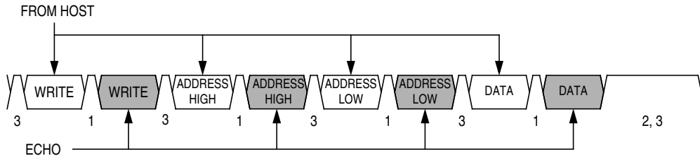
Figure 7-4. Read Transaction
