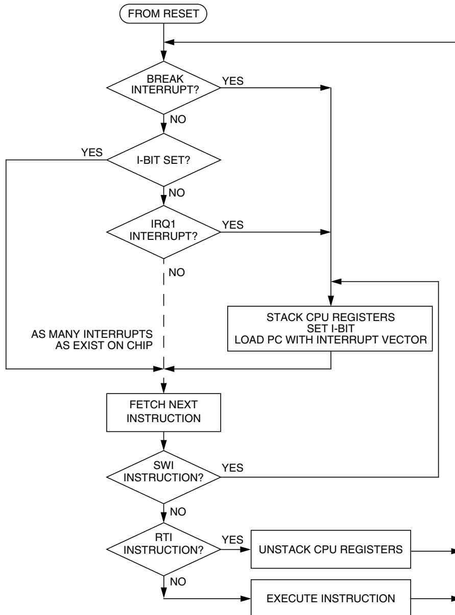
Figure 6-10. Interrupt Processing
