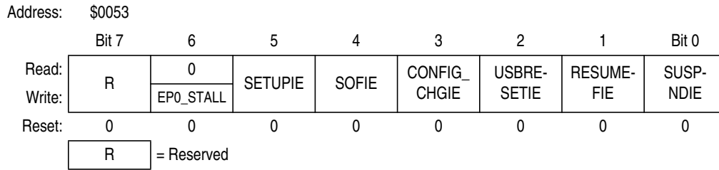
Figure 11-5. USB Status Interrupt Mask Register
