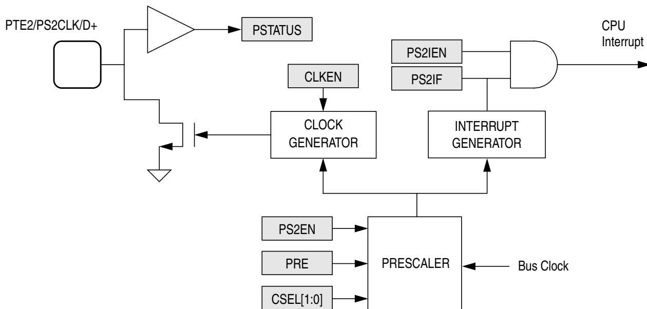
Figure 12-1. PS2 Clock Generator Block Diagram
