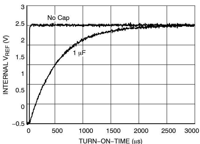
Figure 15. Internal V REF vs. Turn-ON Time
