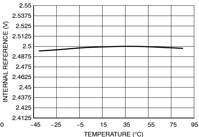
Figure 11. Internal V REF vs. Temperature
